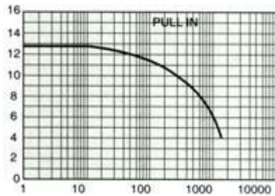
PULSE RATE(Hz) 45BF005-2
