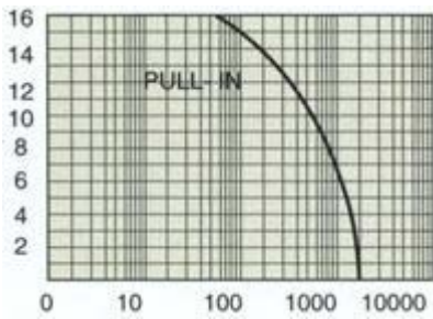
PULSE RATE(Hz) 45BF006
