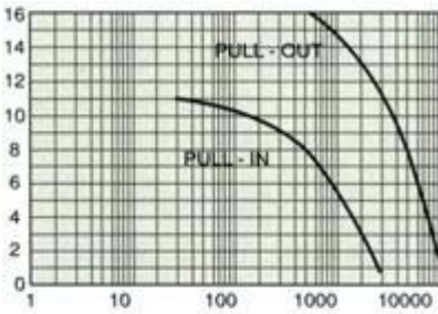
PULSE RATE(Hz) 45BF003-1
