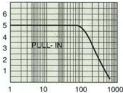
PULSE RATE(Hz) 55BF001
