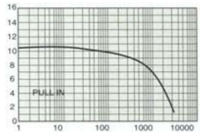
PULSE RATE(Hz) 45BF005-3
