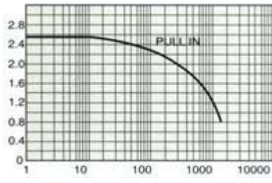
PULSE RATE(Hz) 36BF002-2
